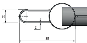
C-C (1:1)
